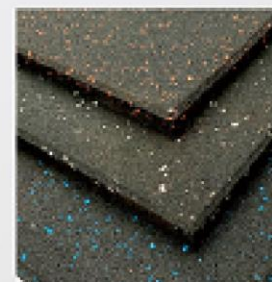
SCL-GP41 EPDM granules surface, bigger SBR granules bottom
